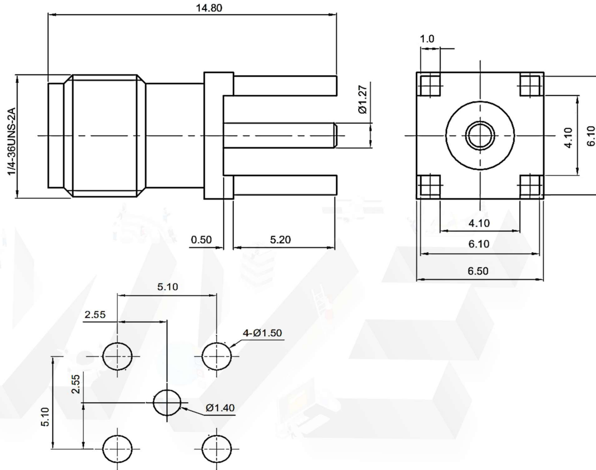
Recommended Mounting Hole
