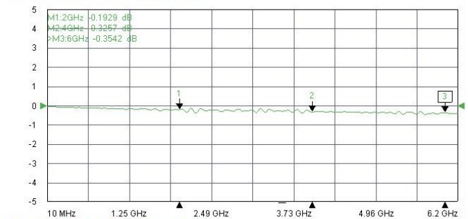
Tr2 S12 Trans LogM RefLvl: 0 dB Res: 1 dB/Div
