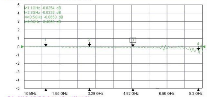
Tr4 S22 Refl SWR RefLvl: 1 U Res: 100 mUIDiv
