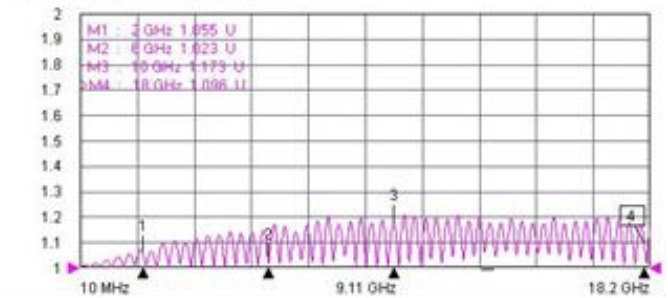
Tr4: S22 Refl SWR RefLvl: 1 U Res: 100 mV/Div
