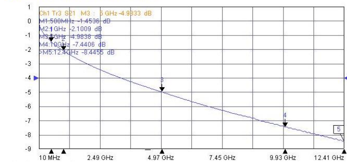
Tr3 S21 Trans LogM RefLvl: -4 dB Res: 1 dB/Div
