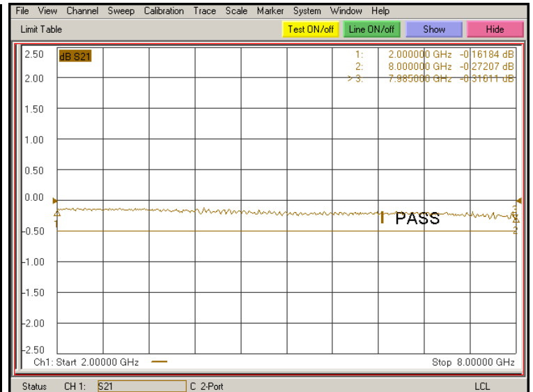
Insertion Loss
